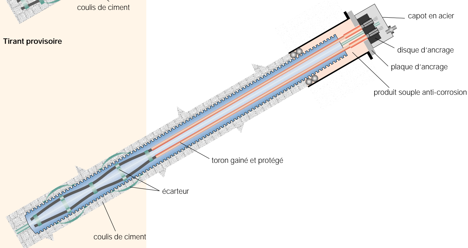
Tirant permanent (DCP)
